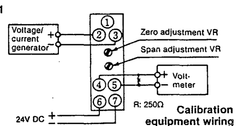
Wiring diagram
