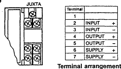
Terminal arrangement
