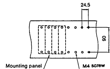
Panel (wall) mounting dimensions
